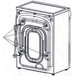
Transit bolts
